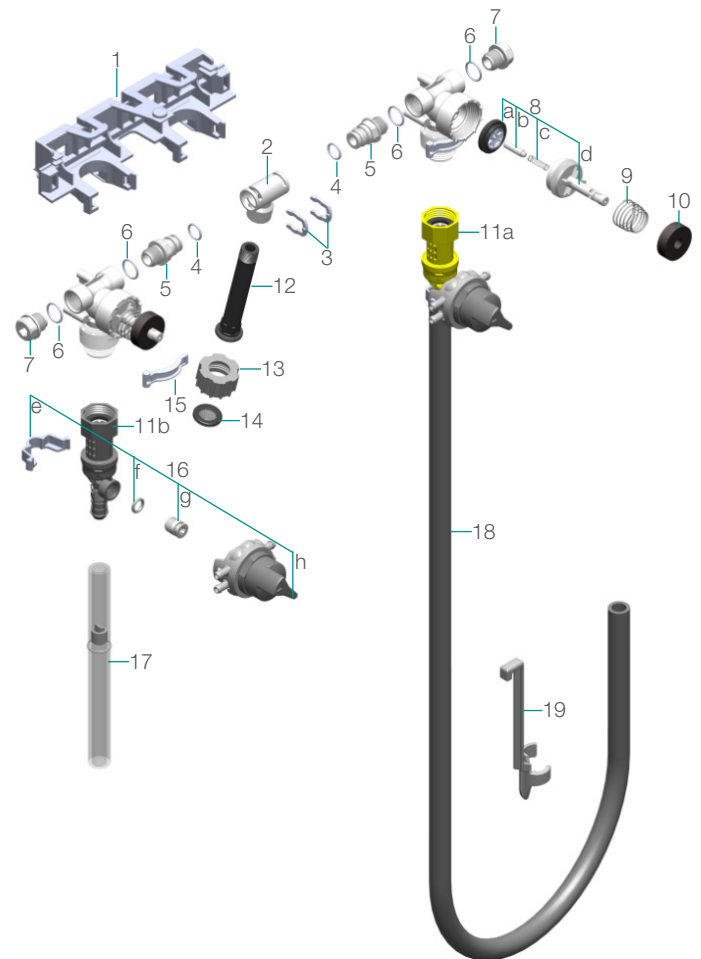
Dual Pick-up
