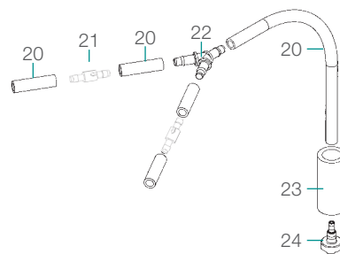
Dual Pick-up
